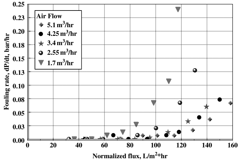
Fig. 2. Fouling rate dP/dt vs. permeate flux J_{20} at different aeration rate in the 2# tube.
